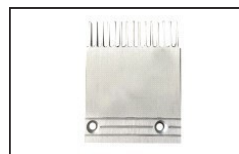
HTAC008 ID:21502024A/C Comb AL L126mm W153mm Hole Space 90mm LHS&CTR 15T
