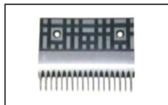
OTAC029 ID:OE-5B 453Y2 Comb AL L139.7mm W108mm Hole Space 101mm 16T
