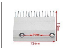
HTAC005 ID:22501790B Comb AL L126mm W112mm Hole Space 90mm CTR 15T
