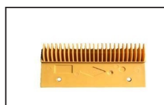
OTPC011 ID:LDTJ-B-2 Comb Plastic L213mm W108mm Hole Space 143mm LHS 25T
