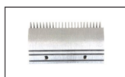
OTAC021 ID:XAA453BJ2 Comb AL L198mm W132.64mm Hole Space 101.7mm RHS 23T
