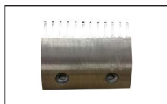
LSAC002 ID:2L08785A Comb AL L108mm W100mm Hole Space 60mm CTR 12T
