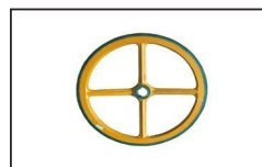
LSFW001 Friction Wheel OD610mm/458mm W45mm ID35mm
