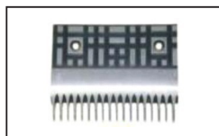
OTAC031 ID:OE-5D 453Y4 Comb AL L145.05mm W108mm Hole Space 101mm 17T
