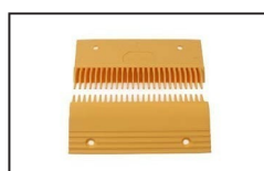
OTPC009 ID:XAA453C2 L47312017A&B Comb Plastic L213mm W108mm Hole Space 142mm LHS 25T
