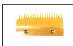
LSPC005 ID: DSA2000168-L ABS Comb L163mm W95mm Hole Space 90mm LHS 19T
