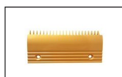
OTPC001 ID:L47312022A ABS Comb L204mm W107mm Hole Space 145mm RHS 22T
