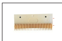
OTPC005 ID:L47312018AB Comb Plastic L212mm W108mm Hole Space 145mm LHS 25T
