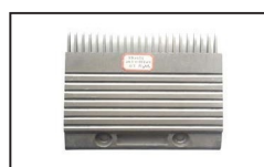
KOAC015 ID:DEE3703288 Comb AL L200.7mm W178.8mm Hole Space 99mm RHS 22T
