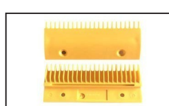
LSPC012 ID: DSA2001489-M ABS Comb L199mm W93.5mm Hole Space 119mm CTR 22T
