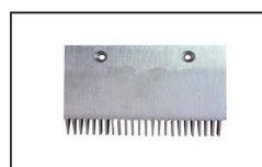
LSAC007 ID:DSA2000905-B Comb AL L206mm W139mm Hole Space 110mm LHS 24T
