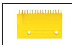
HTPC016 ID:2507223-B Comb Plastic L147mm W90mm Hole Space 90mm LHS 17T
