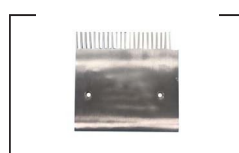
HDAC007-2 ID: P9.068 S655C942H02 Comb AL L207mm W193mm Hole Space 145mm RHS 22T
