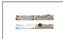
LSLP012 Landing Door Hanger Plate L455mm W140mm
