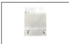
HTAC007 ID:21502024B/D Comb AL L126mm W153mm Hole Space 90mm CTR&RHS 15T
