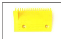
HTPC009 ID:C0036728B GN525 Comb Plastic L150mm W93mm Hole Space 90mm LHS 17T
