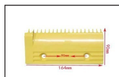
HTPC004 ID:H2200146 Comb Plastic L164mm W90mm Hole Space 90mm LHS 19T
