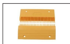
OTPC008 ID:XAA453C3 L47312018A&B Comb Plastic L213mm W108mm Hole Space 142mm RHS 25T
