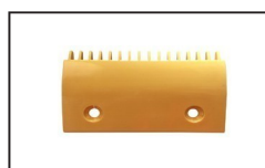
LS0C001 ID: 2L08316 ABS Comb L145mm W90mm Hole Space 90mm CTR 16T
