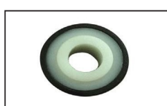
KOLR017 ID:KM359391G01 Door Lock Roller OD31.5mm ID12mm
