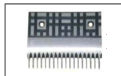
OTAC032 ID:OE-5 453Y5 Comb AL L137.16mm W108mm Hole Space 101mm 16T
