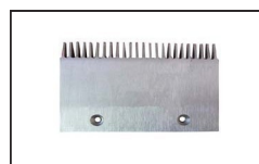
LSAC005 ID:DSA2000903-B Comb AL L203mm W139mm Hole Space 110mm CTR 24T
