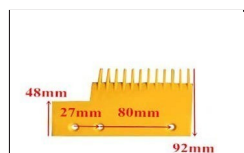
HDPC008 ID:S655B6 ABS Comb Yellow L155mm W92mm Hole Space 80/27mm LHS 12T
