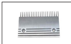
TOAC001-2 Comb AL L199mm W130mm Hole Space 145mm CTR 22T
