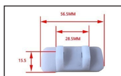
OTNC019 ID:DAA180JM3 Newel Chain Accessory
