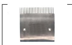
HDAC007-1 ID: P9.068 S655C942H01 Comb AL L200mm W193mm Hole Space 145mm CTR 22T
