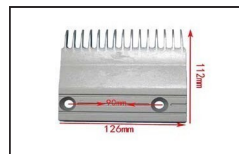
HTAC004 ID:22501790A Comb AL L126mm W112mm Hole Space 90mm CTR 15T
