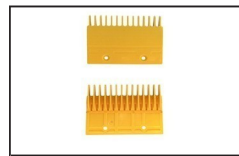
MIPC004 ID:YS120B976 Comb Plastic L127mm W97mm Hole Space 64mm CTR 14T
