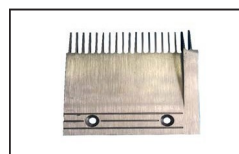
HTAC010 ID:21502025A/B Comb AL L164mm W153mm Hole Space 90mm RHS 19T
