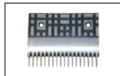
OTAC030 ID:OE-5C 453Y3 Comb AL L144.78mm W108mm Hole Space 101mm 17T
