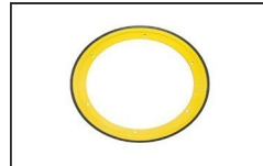
OTFW032 OD557mm W30mm ID433mm Friction Wheel
