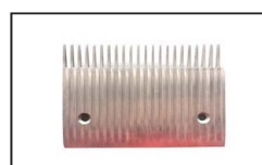
SCAC011 ID:SFR247416 DAW-A305004N Comb AL L199mm W154mm Hole Space 145mm RHS/CTR 22T
