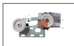
SCLP122 ID:59305577 Landing Door Lock LHS for V50
