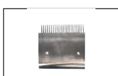
HDAC007-3 ID: P9.068 S655C942H03 Comb AL L213mm W193mm Hole Space 145mm LHS 22T
