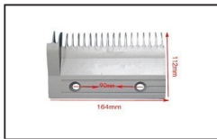
HTAC001 ID:22501787A Comb AL L164mm W112mm Hole Space 90mm LHS 19T
