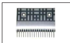
OTAC033 ID:OE-5E 453Y6 Comb AL L142.24mm W108mm Hole Space 101mm 17T
