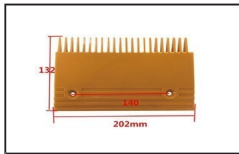
KOPC002 ID:KM5009371H02 Comb L202mm W132mm Hole Space 140mm RHS 22T
