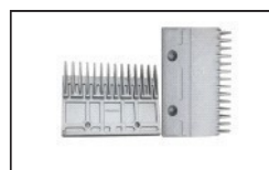
MIAC005 ID:J651004B203 Comb AL L126mm W90mm Hole Space 64mm 14T
