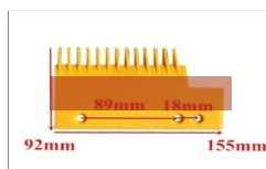
HDPC009 ID:S655B6 ABS Comb Yellow L155mm W92mm Hole Space 89/18mm RHS 13T
