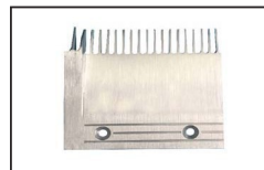
HTAC006 ID:21502026A/B Comb AL L164mm W153mm Hole Space 90mm LHS 19T
