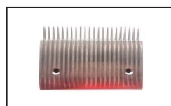
SCAC012 ID:SFR247417 DAW-A305004N Comb AL L205mm W154mm Hole Space 145mm LHS 22T
