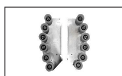
SCRL031 Handrail Roller Assy Roller OD70mm W50mm 6204-2RS
