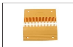
OTPC007 ID:XAA453C1 L57312013 Comb Plastic L191mm W108mm Hole Space 142mm CTR 23T
