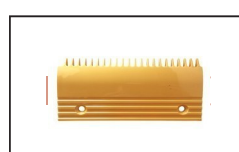
OTPC003 ID:L47312024A ABS Comb L204mm W107mm Hole Space 145mm LHS 22T
