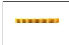
LSDM003 ID:2L05913-M Demarcation L318mm W40mm 38T
